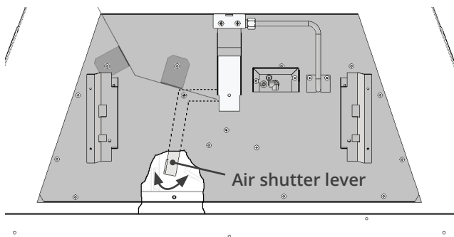
Top view—cut out shows the air shutter lever located under the module plate.
