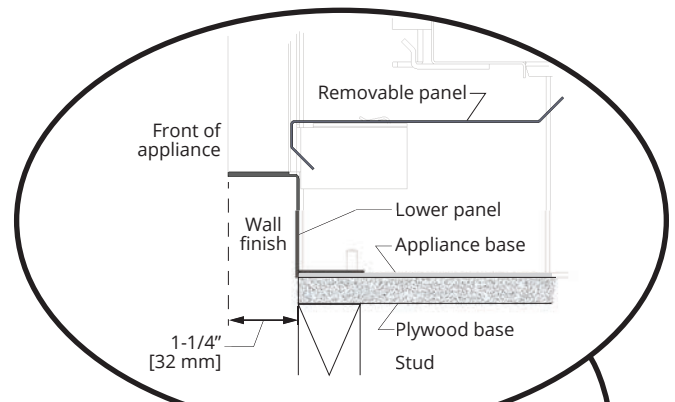
Section view, up the wall—detail
